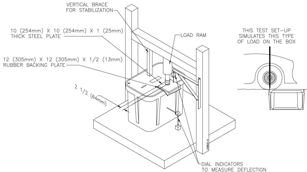
Figure 8 - Box Vertical Sidewall Load Test (Pedestrian, Tiers 5, 8 & 15)
